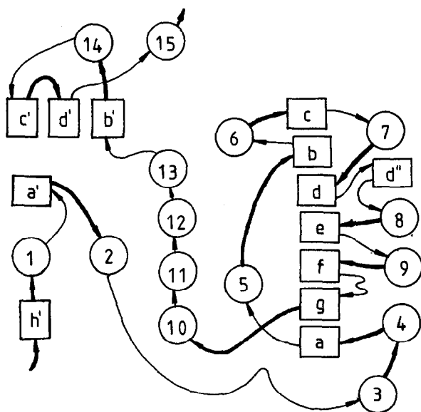
Fig.1. Topology-packing diagram of a subunit of cAATase. \alpha -Helices and \beta -strands are denoted as in [4]: (○) helices; (□) \beta -strands.
